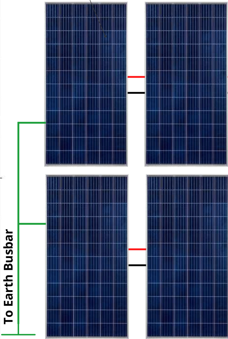
2S-2P Arrangement of Solar panels
